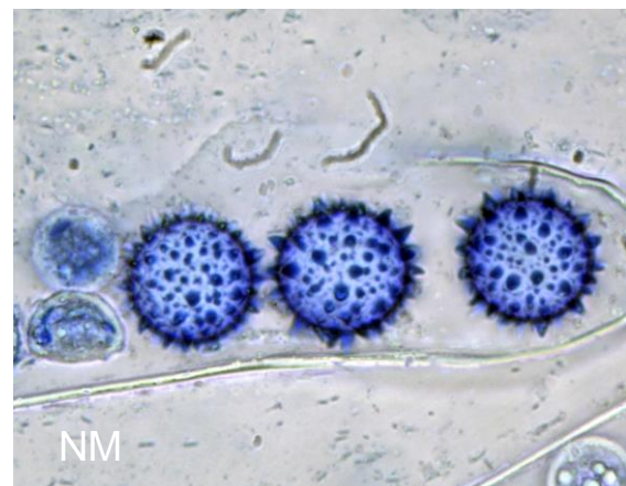
Abb. 8: Derbstacheliger Rundspor-Schildborstling
